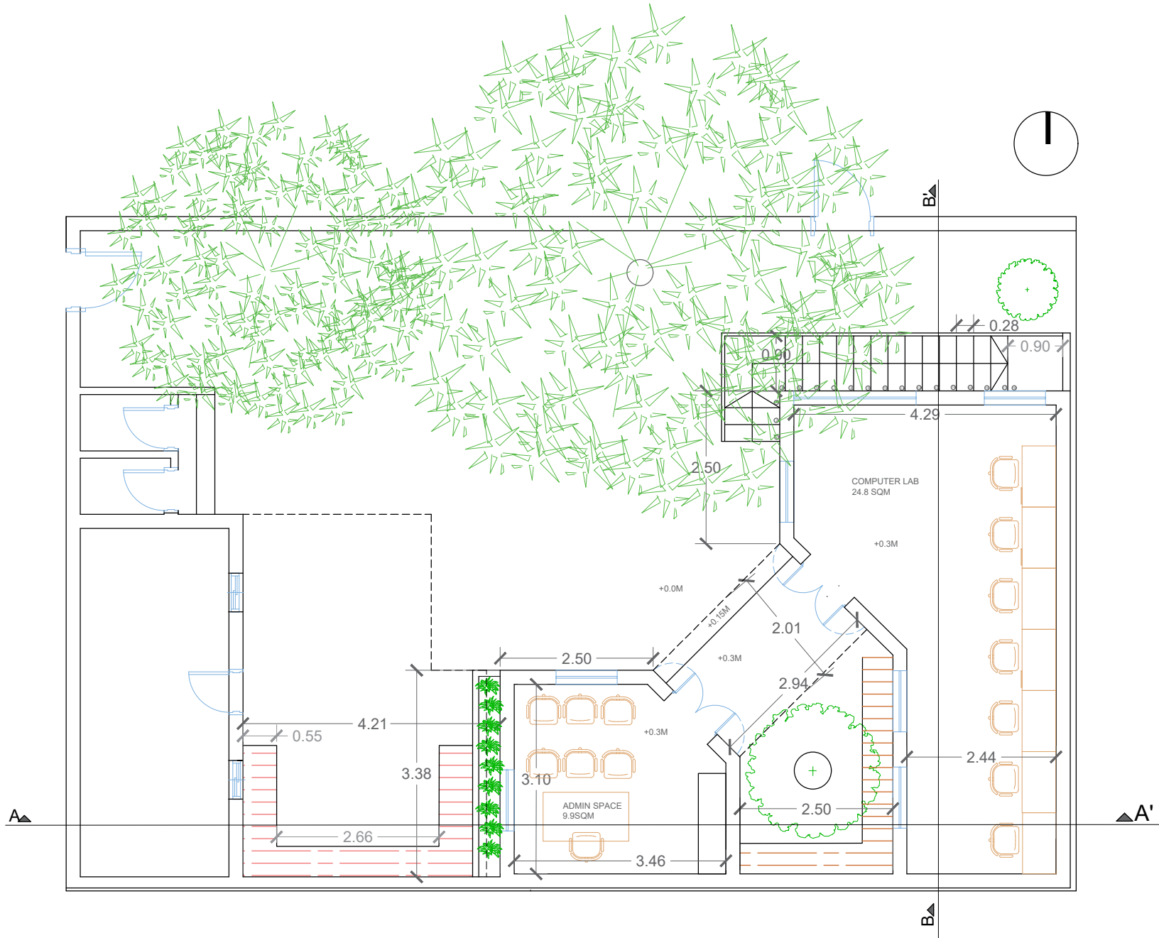
GROUND FLOOR
