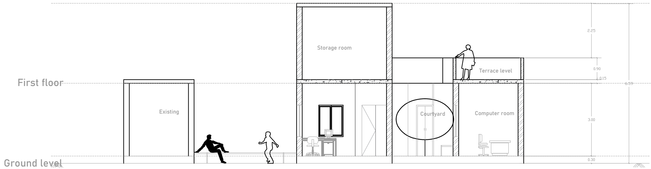
SECTION AA'
