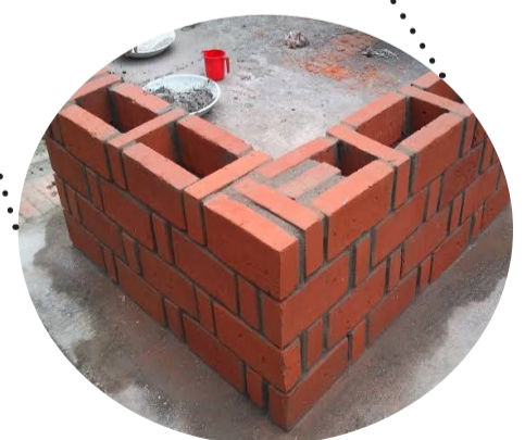
WALLS - RAT TRAP BOND
